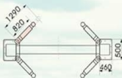
Outline Drawing (Unit:mm)
